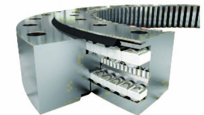
三排滚柱式回转支承 Three-row roller series
